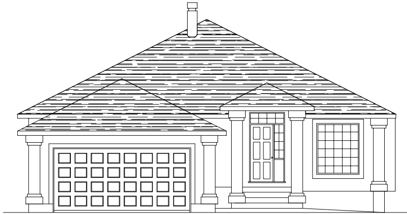
FRONT ELEVATION
